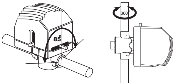
Figure 1. Mounting
