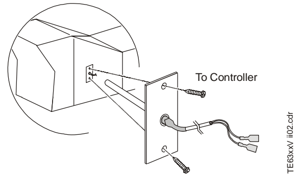
Figure 2: Installing the VAV Duct Probe Sensor
