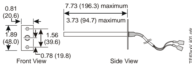
Figure 1: Sensor Dimensions, in. (mm)
